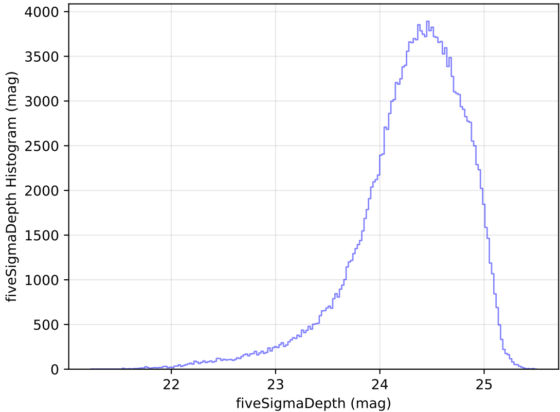
too_elab_heavy_r32_d3_gz_v3.4_10yrs All sky g band: fiveSigmaDepth Histogram
