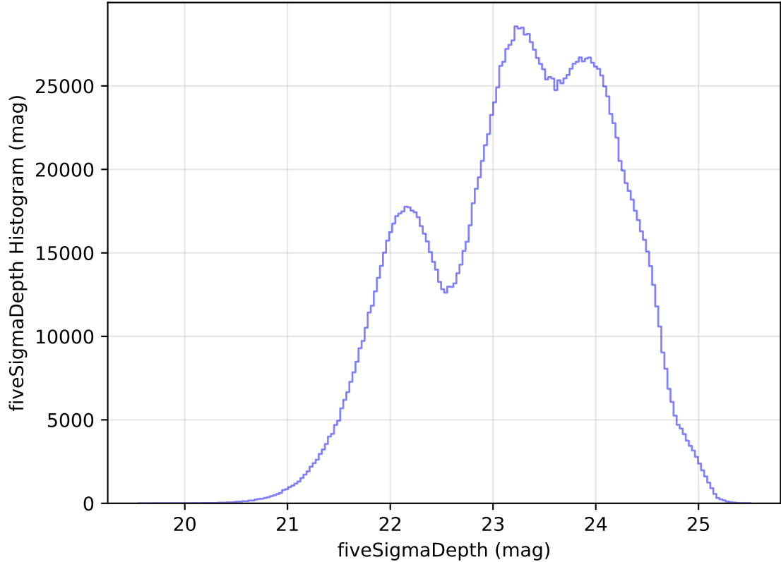
too_elab_heavy_r32_d3_gz_v3.4_10yrs All sky all bands: fiveSigmaDepth Histogram
