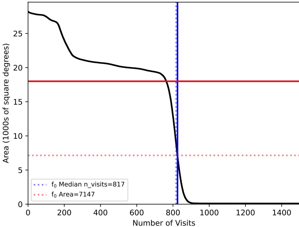
too_elab_heavy_r32_d3_gz_v3.4_10yrs All sky: f0
