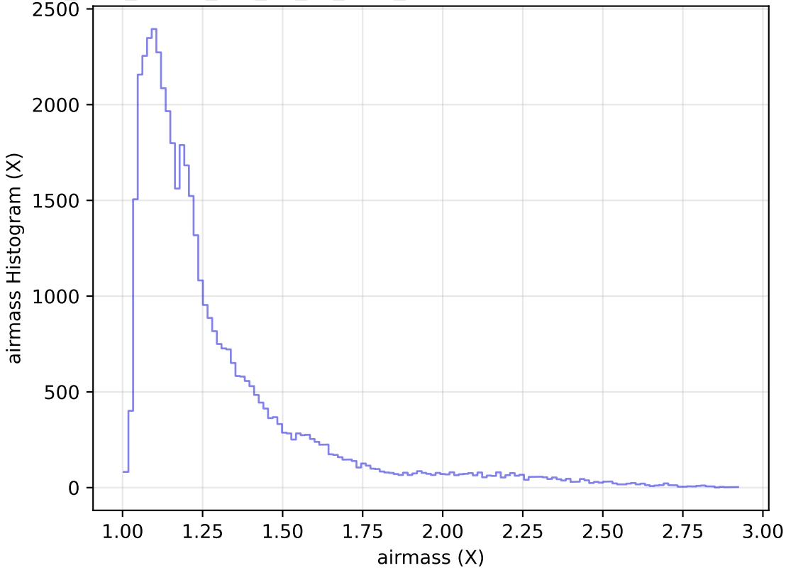
too_elab_heavy_r32_d3_gz_v3.4_10yrs Yr 1 z band: airmass Histogram
