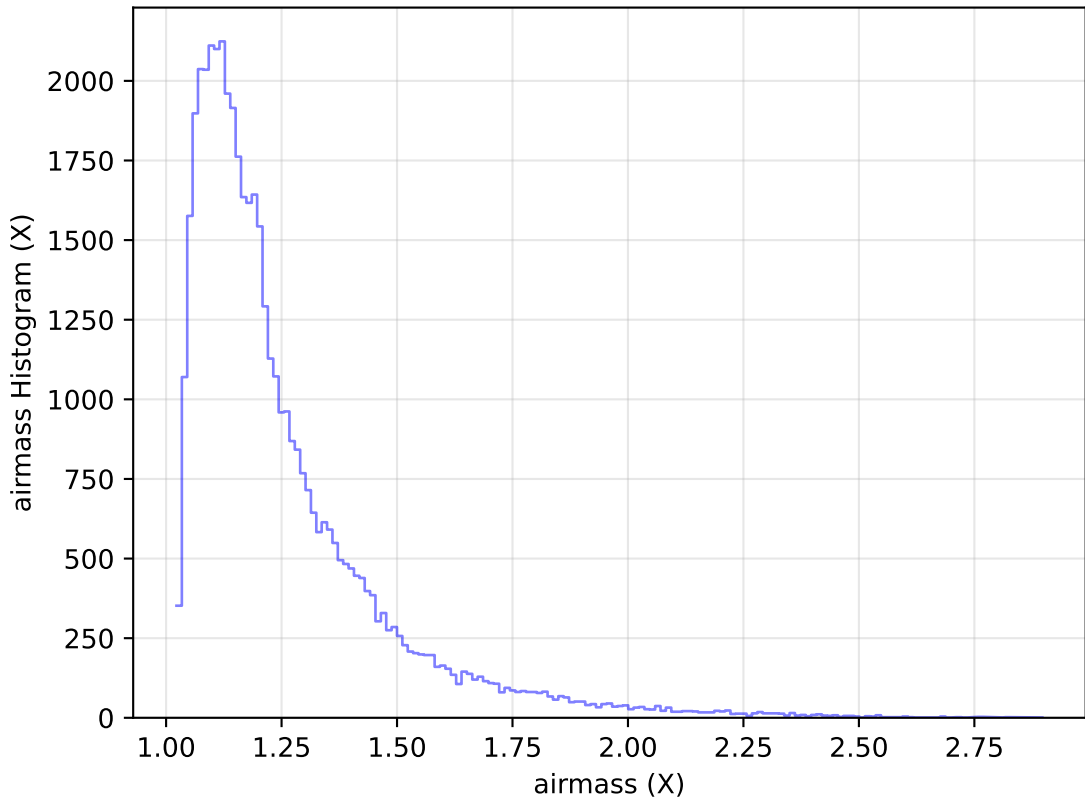
too_elab_heavy_r32_d3_gz_v3.4_10yrs Yr 1 y band: airmass Histogram
