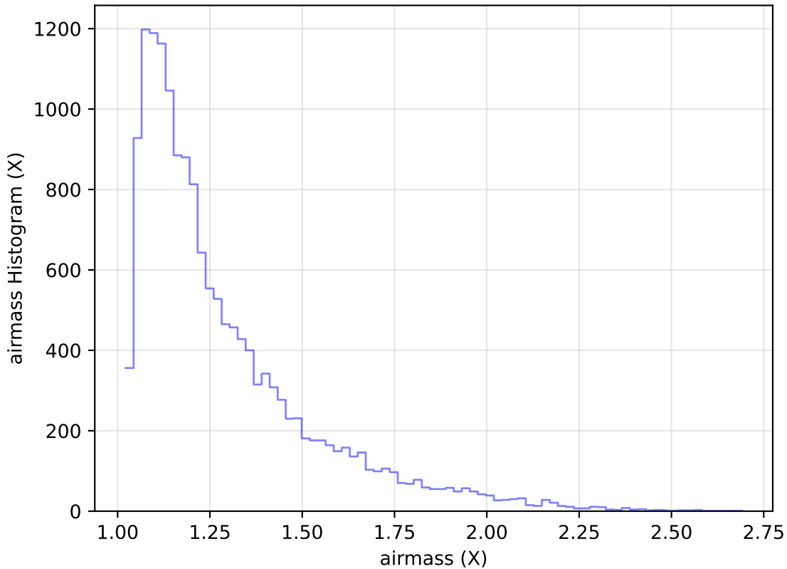
too_elab_heavy_r32_d3_gz_v3.4_10yrs Yr 1 u band: airmass Histogram
