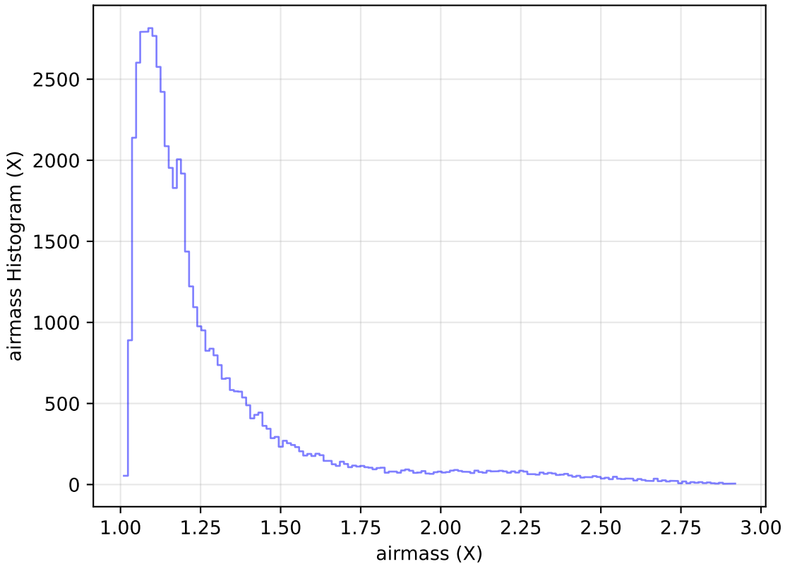
too_elab_heavy_r32_d3_gz_v3.4_10yrs Yr 1 i band: airmass Histogram
