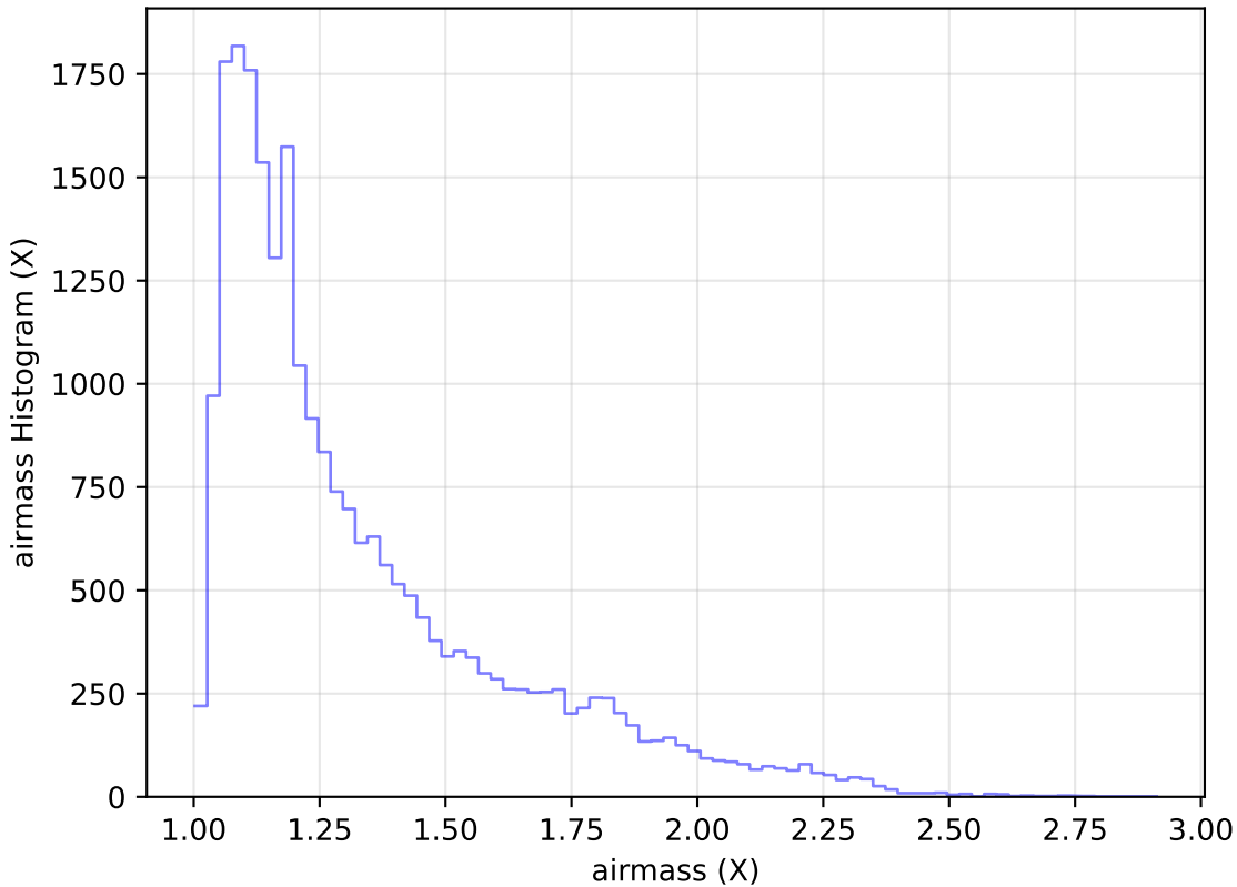
too_elab_heavy_r32_d3_gz_v3.4_10yrs Yr 1 g band: airmass Histogram
