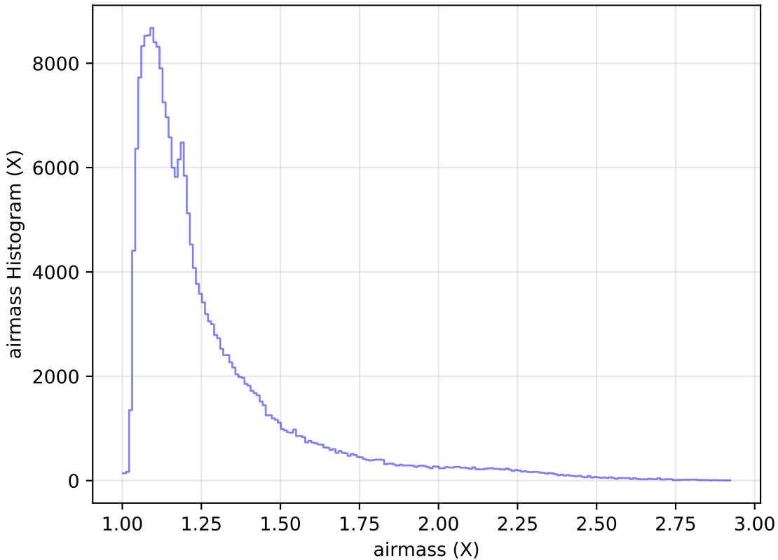
too_elab_heavy_r32_d3_gz_v3.4_10yrs Yr 1 all bands: airmass Histogram
