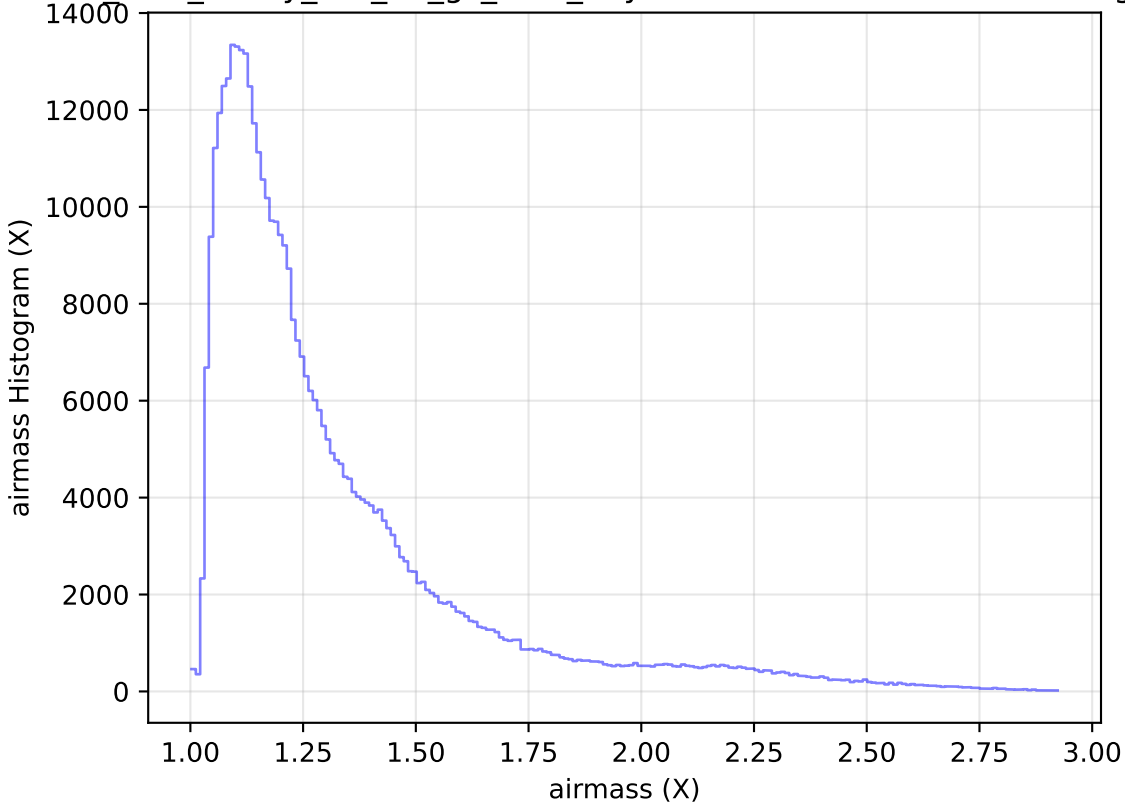
too_elab_heavy_r32_d3_gz_v3.4_10yrs WFD z band: airmass Histogram
