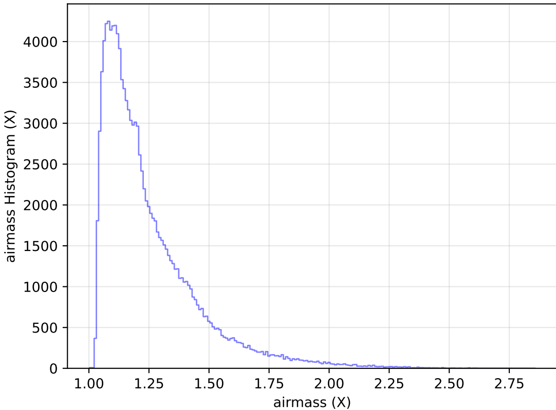
too_elab_heavy_r32_d3_gz_v3.4_10yrs WFD u band: airmass Histogram
