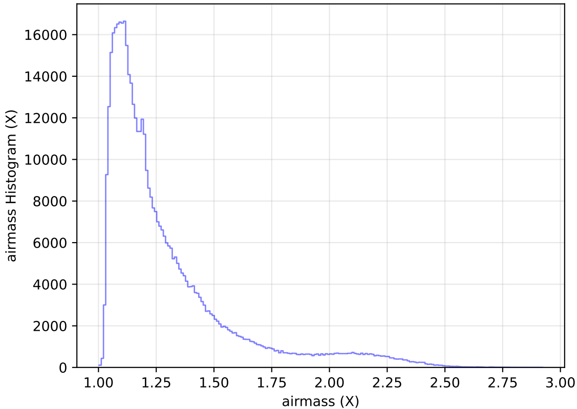
too_elab_heavy_r32_d3_gz_v3.4_10yrs WFD r band: airmass Histogram
