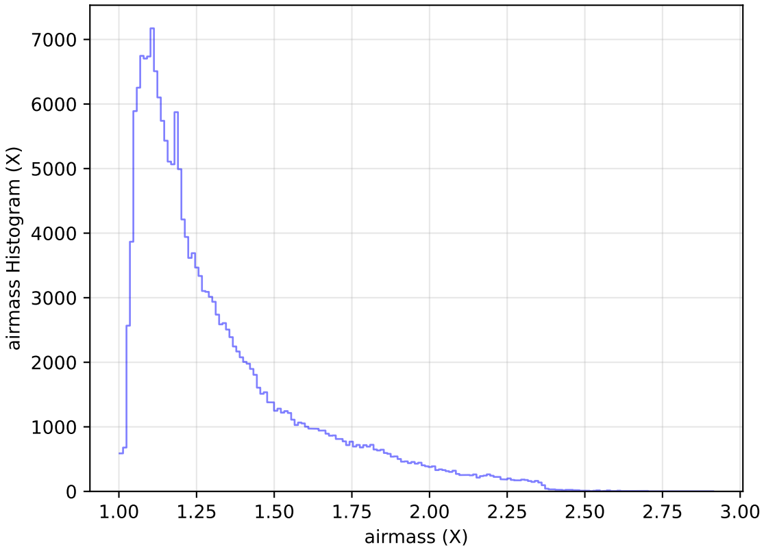
too_elab_heavy_r32_d3_gz_v3.4_10yrs WFD g band: airmass Histogram
