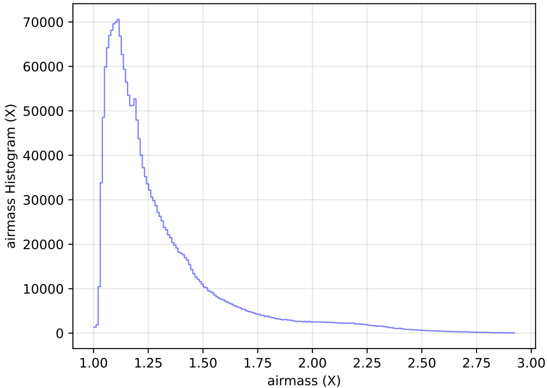
too_elab_heavy_r32_d3_gz_v3.4_10yrs WFD all bands: airmass Histogram
