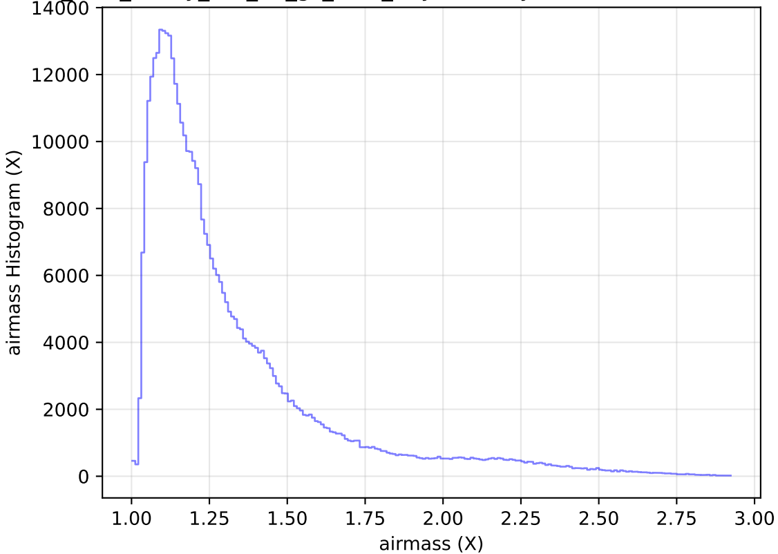
too_elab_heavy_r32_d3_gz_v3.4_10yrs All sky z band: airmass Histogram
