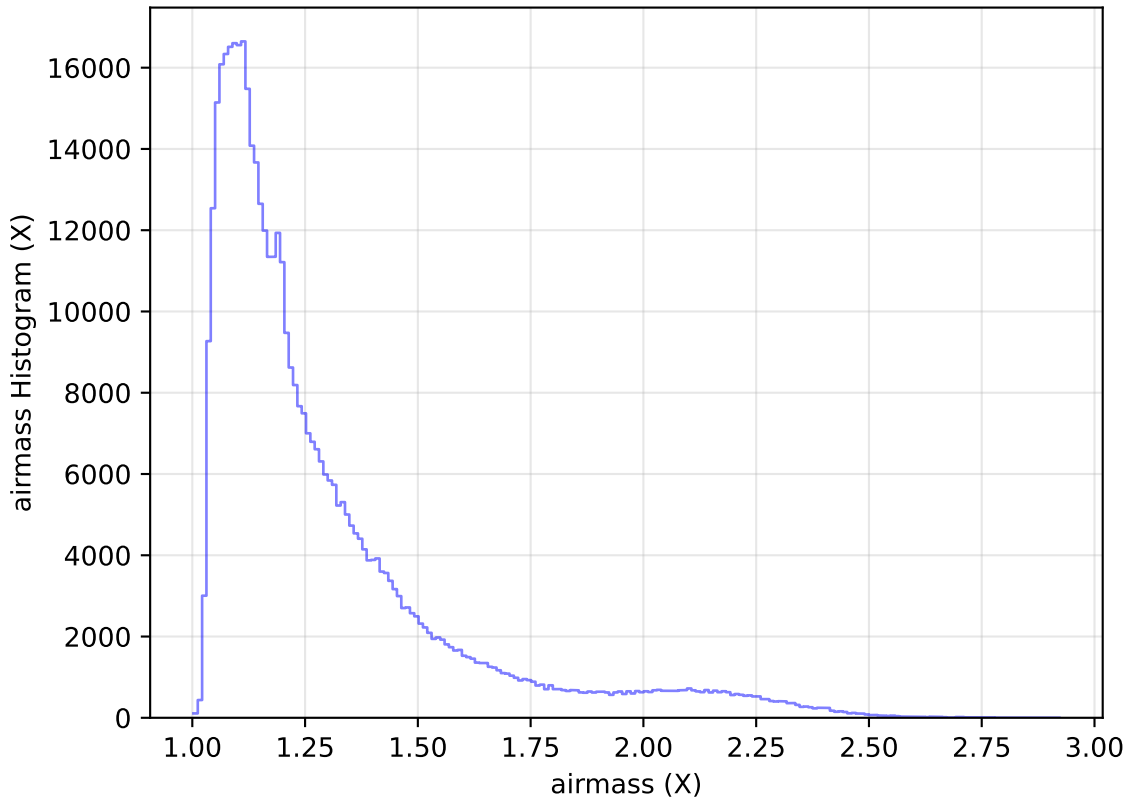
too_elab_heavy_r32_d3_gz_v3.4_10yrs All sky r band: airmass Histogram
