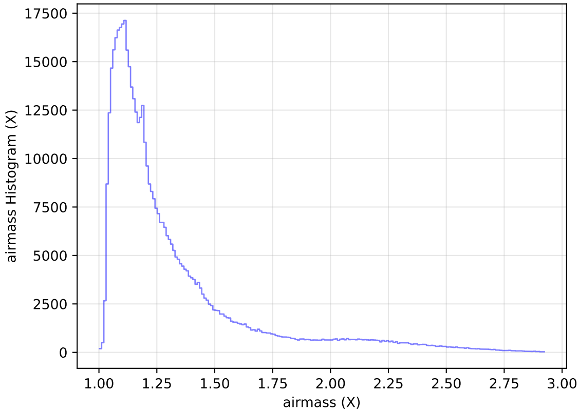
too_elab_heavy_r32_d3_gz_v3.4_10yrs All sky i band: airmass Histogram
