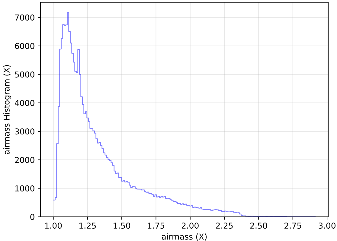
too_elab_heavy_r32_d3_gz_v3.4_10yrs All sky g band: airmass Histogram
