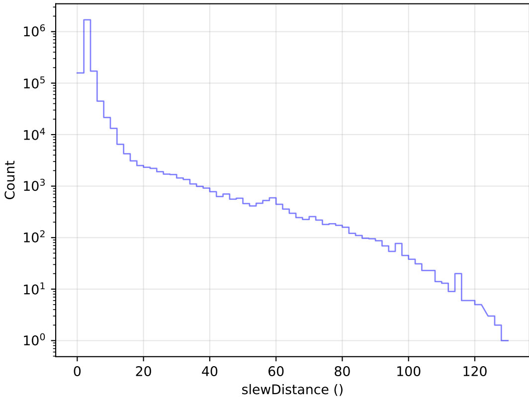
too_elab_heavy_r32_d3_gz_v3.4_10yrs All visits: Slew Distance Histogram
