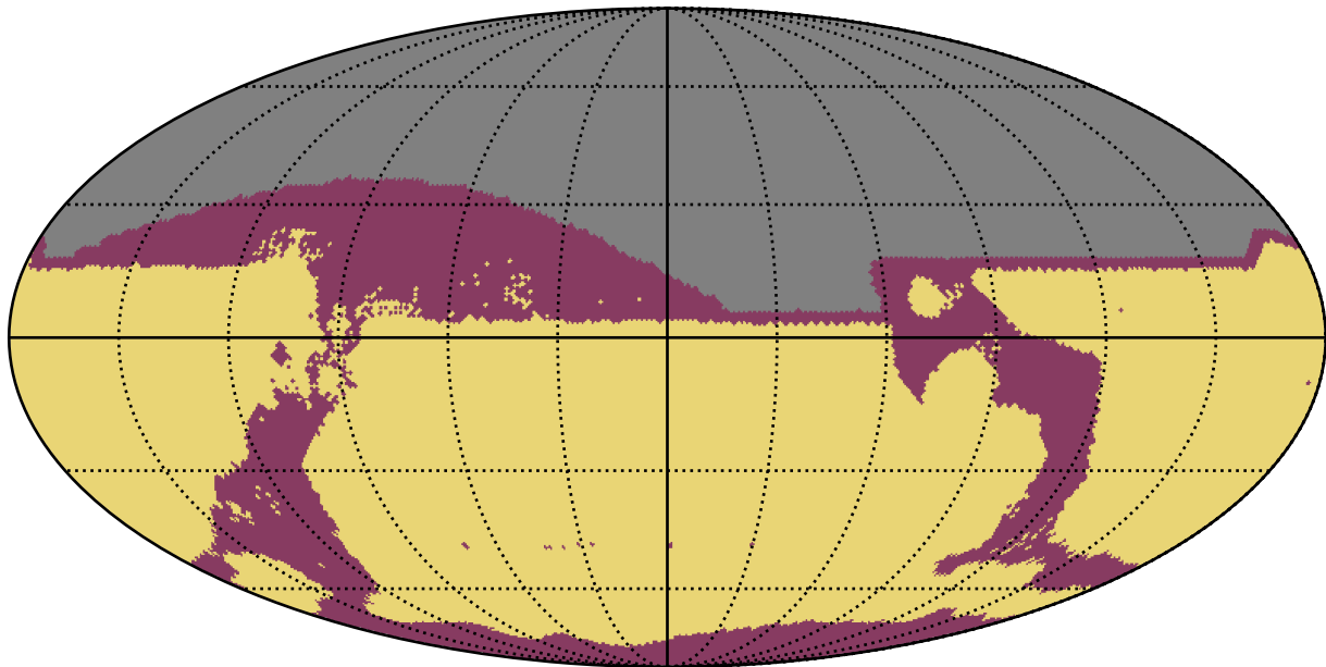
too_elab_heavy_r32_d3_gz_v3.4_10yrs All sky: RapidRevisits
