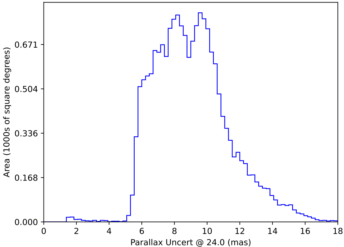
too_elab_heavy_r32_d3_gz_v3.4_10yrs WFD: Parallax Uncert @ 24.0
