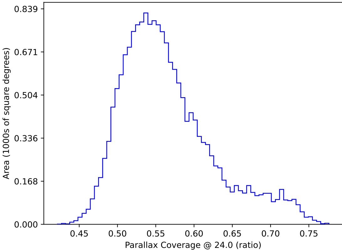
too_elab_heavy_r32_d3_gz_v3.4_10yrs WFD: Parallax Coverage @ 24.0
