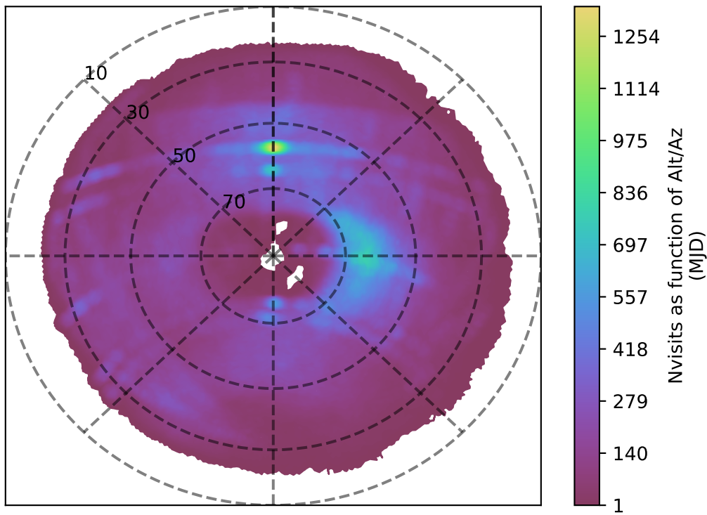
too_elab_heavy_r32_d3_gz_v3.4_10yrs g band: Nvisits as function of Alt/Az
