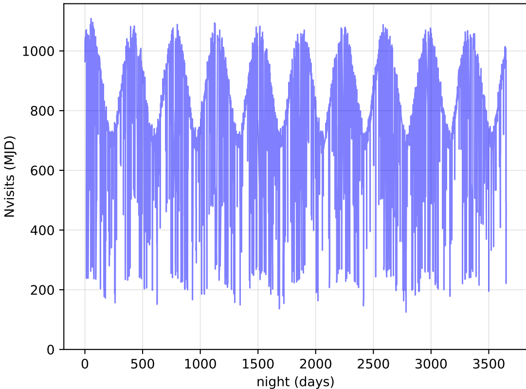
too_elab_heavy_r32_d3_gz_v3.4_10yrs All visits: Nvisits
