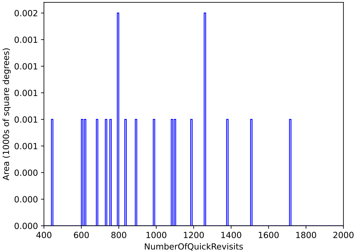
too_elab_heavy_r32_d3_gz_v3.4_10yrs All sky: NumberOfQuickRevisits
