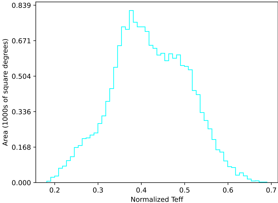
too_elab_heavy_r32_d3_gz_v3.4_10yrs WFD u band: Normalized Teff
