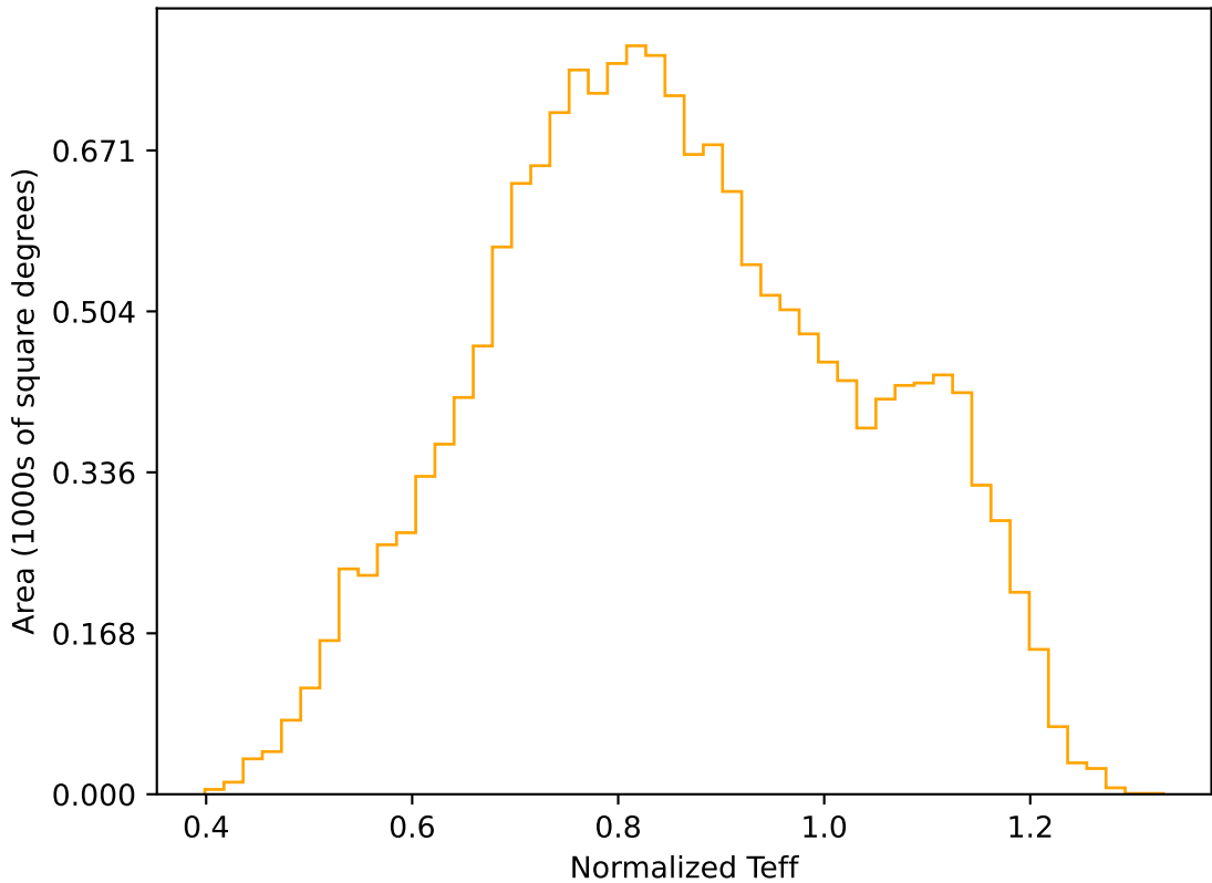
too_elab_heavy_r32_d3_gz_v3.4_10yrs WFD r band: Normalized Teff
