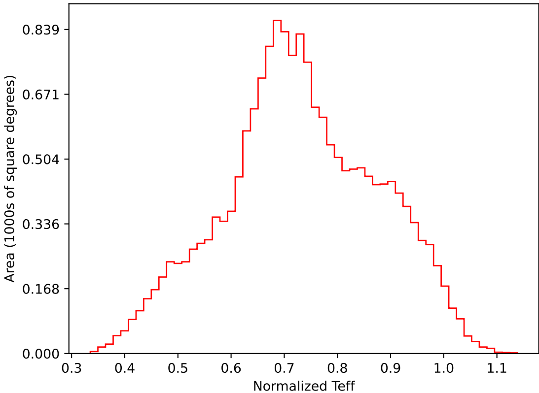
too_elab_heavy_r32_d3_gz_v3.4_10yrs WFD i band: Normalized Teff
