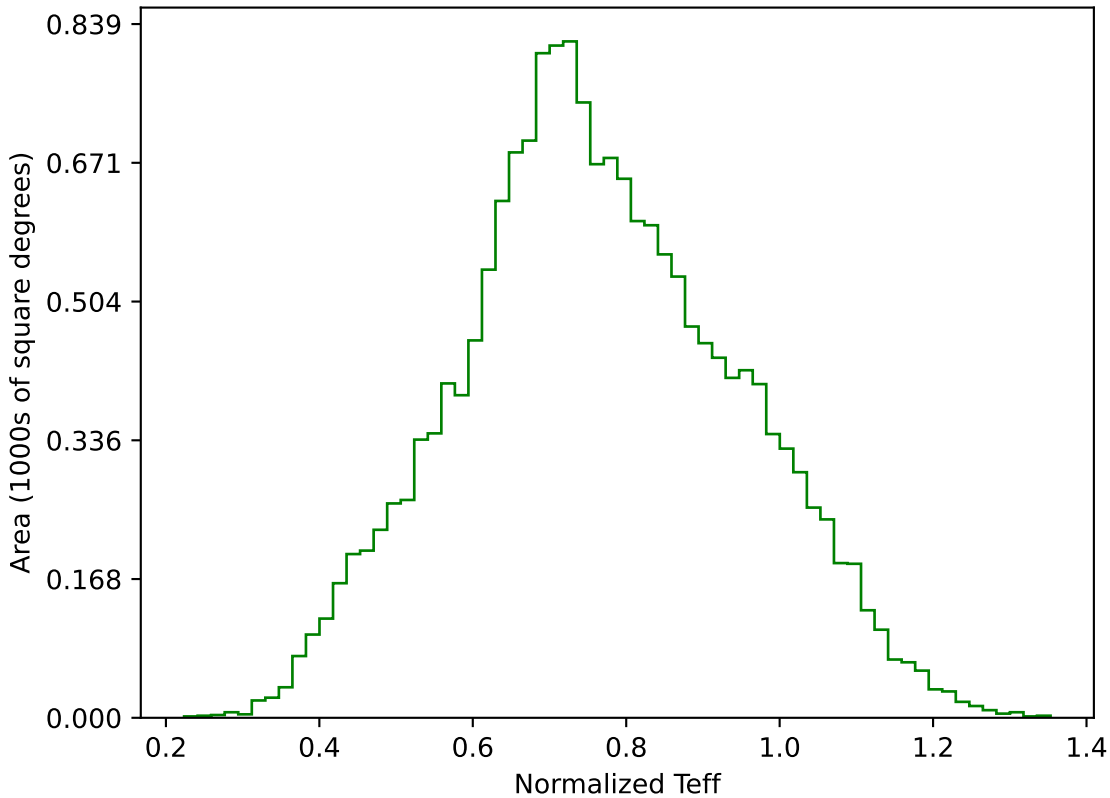
too_elab_heavy_r32_d3_gz_v3.4_10yrs WFD g band: Normalized Teff
