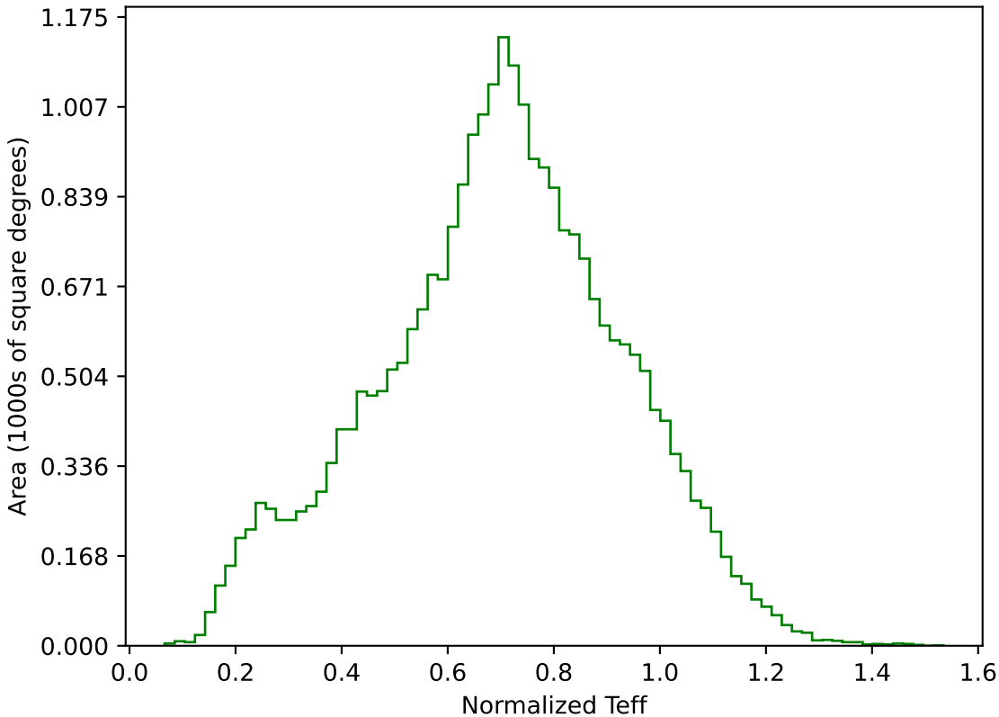
too_elab_heavy_r32_d3_gz_v3.4_10yrs All sky g band: Normalized Teff
