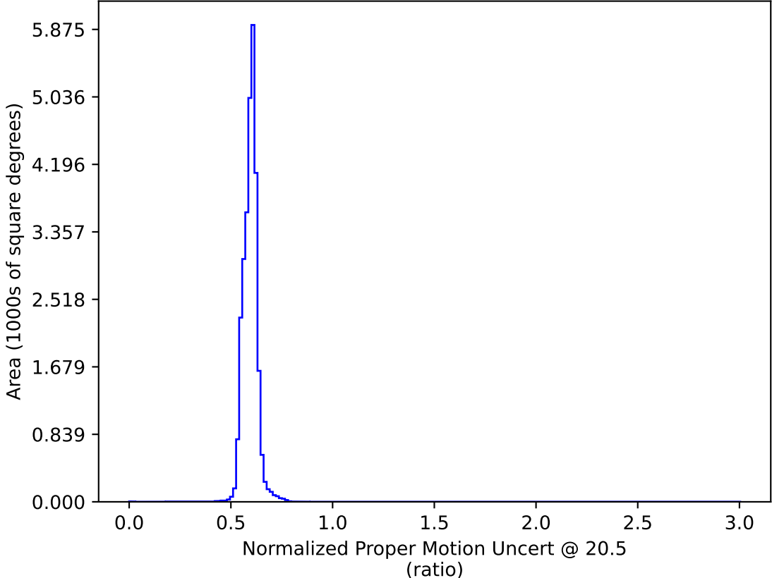
too_elab_heavy_r32_d3_gz_v3.4_10yrs All sky: Normalized Proper Motion Uncert @ 20.5
