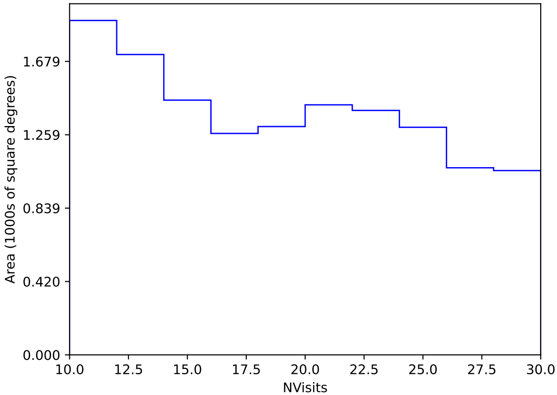
too_elab_heavy_r32_d3_gz_v3.4_10yrs Yr 3-4 y band: NVisits
