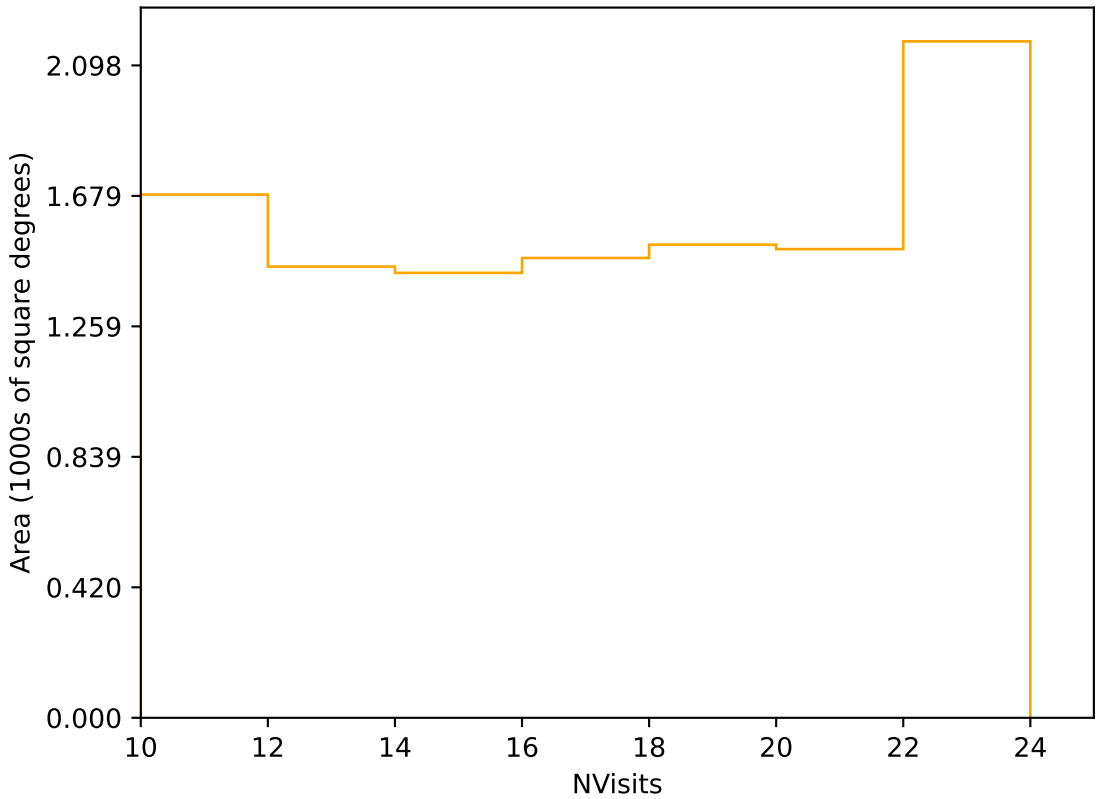
too_elab_heavy_r32_d3_gz_v3.4_10yrs Yr 3-4 r band: NVisits
