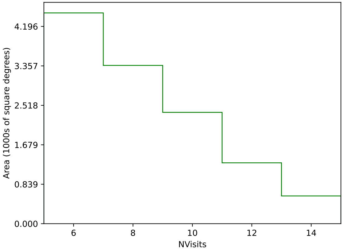
too_elab_heavy_r32_d3_gz_v3.4_10yrs Yr 3-4 g band: NVisits
