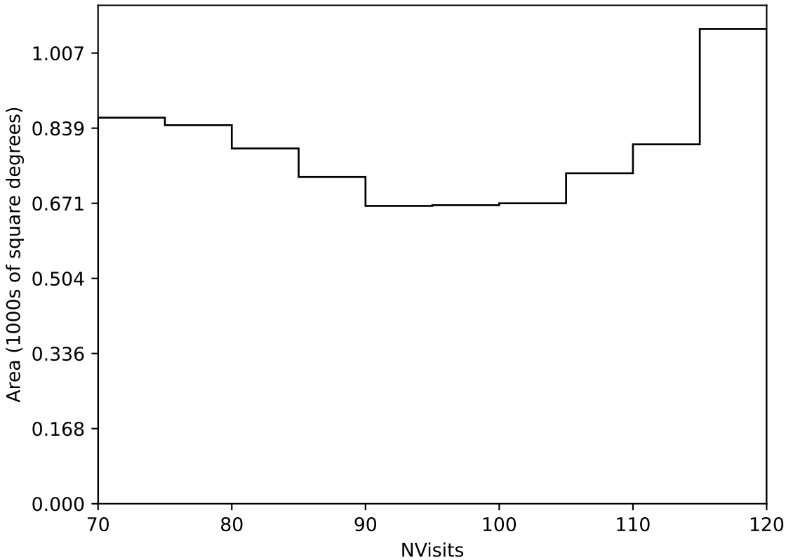
too_elab_heavy_r32_d3_gz_v3.4_10yrs Yr 3-4 all bands: NVisits
