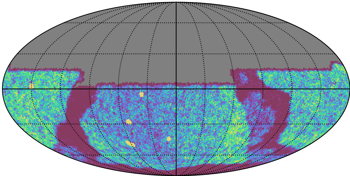
too_elab_heavy_r32_d3_gz_v3.4_10yrs Yr 1 y band: NVisits
