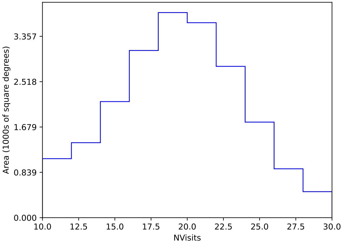
too_elab_heavy_r32_d3_gz_v3.4_10yrs Yr 1 y band: NVisits
