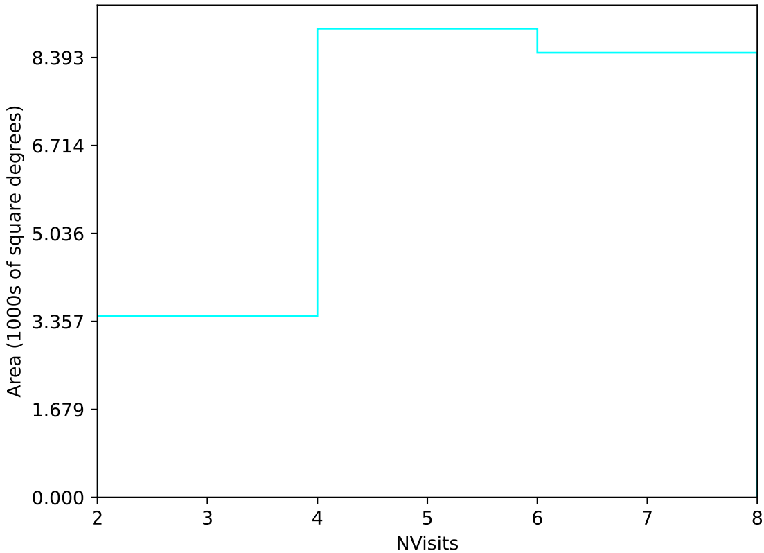
too_elab_heavy_r32_d3_gz_v3.4_10yrs Yr 1 u band: NVisits
