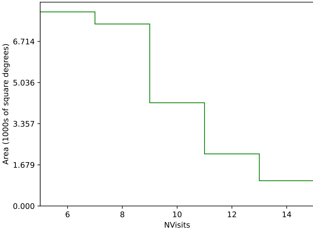
too_elab_heavy_r32_d3_gz_v3.4_10yrs Yr 1 g band: NVisits
