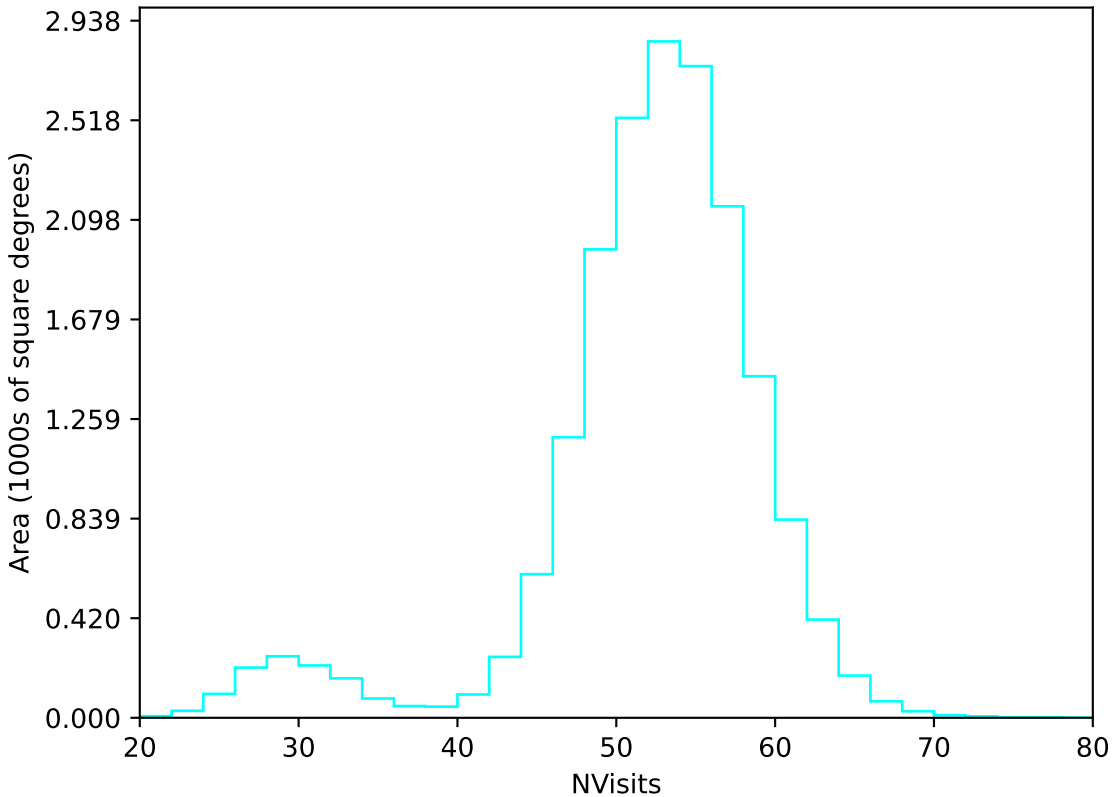
too_elab_heavy_r32_d3_gz_v3.4_10yrs WFD u band: NVisits
