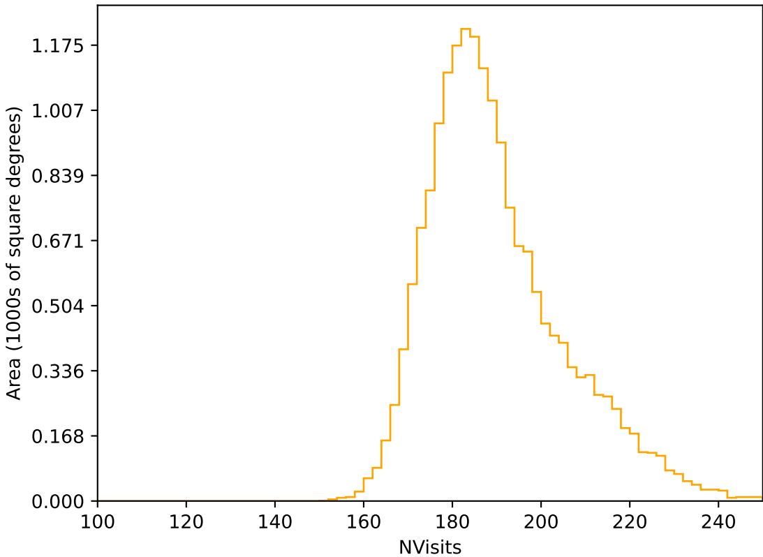
too_elab_heavy_r32_d3_gz_v3.4_10yrs WFD r band: NVisits
