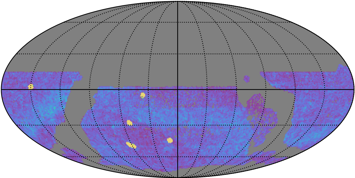
too_elab_heavy_r32_d3_gz_v3.4_10yrs WFD all bands: NVisits
