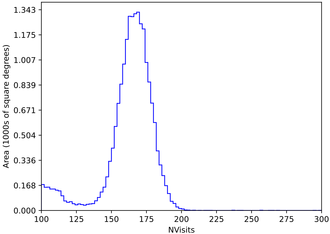
too_elab_heavy_r32_d3_gz_v3.4_10yrs All sky y band: NVisits
