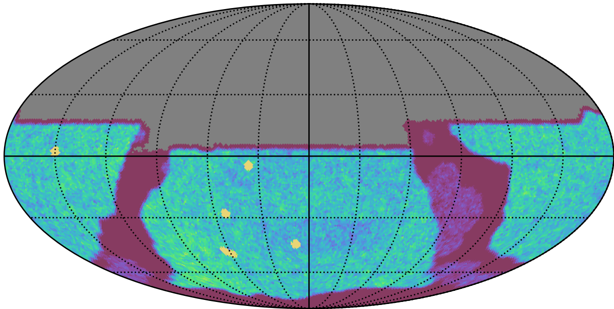
too_elab_heavy_r32_d3_gz_v3.4_10yrs All sky u band: NVisits
