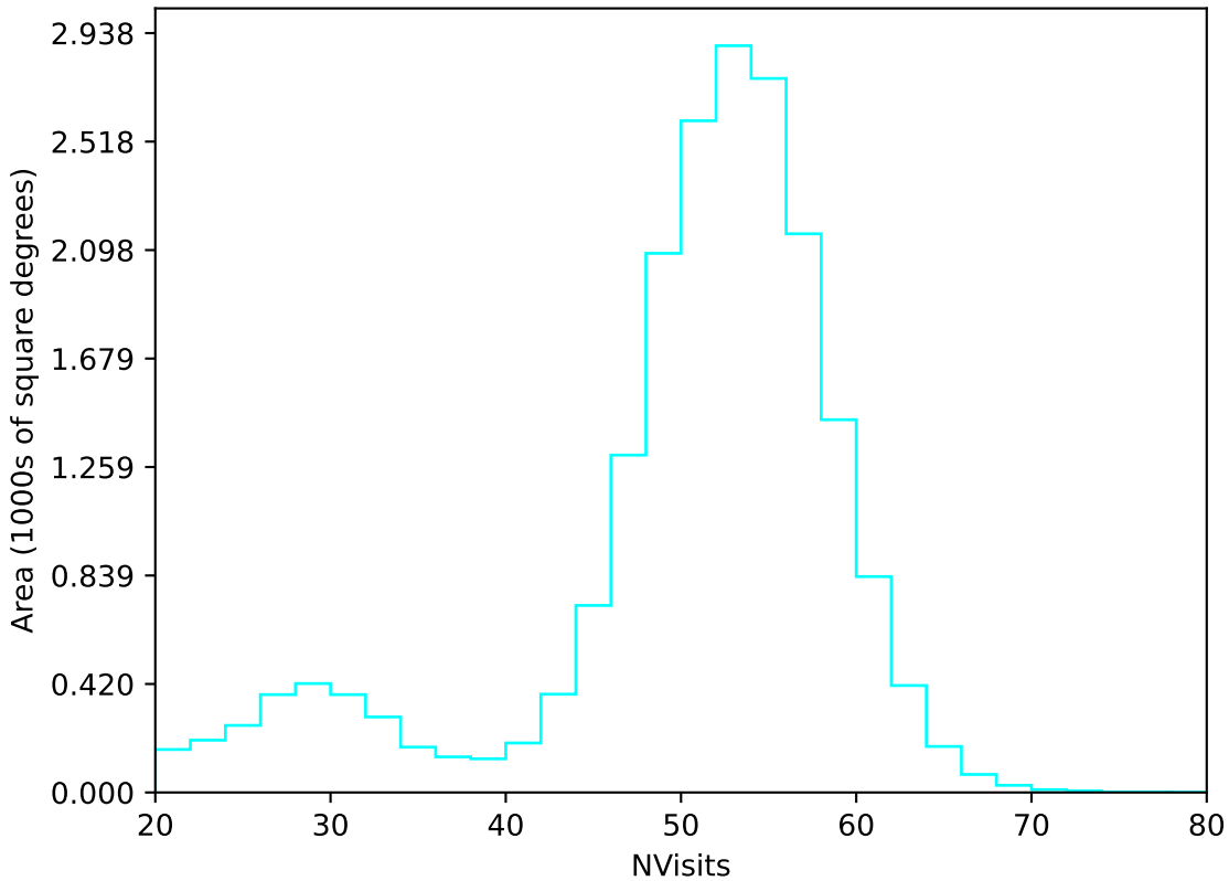
too_elab_heavy_r32_d3_gz_v3.4_10yrs All sky u band: NVisits
