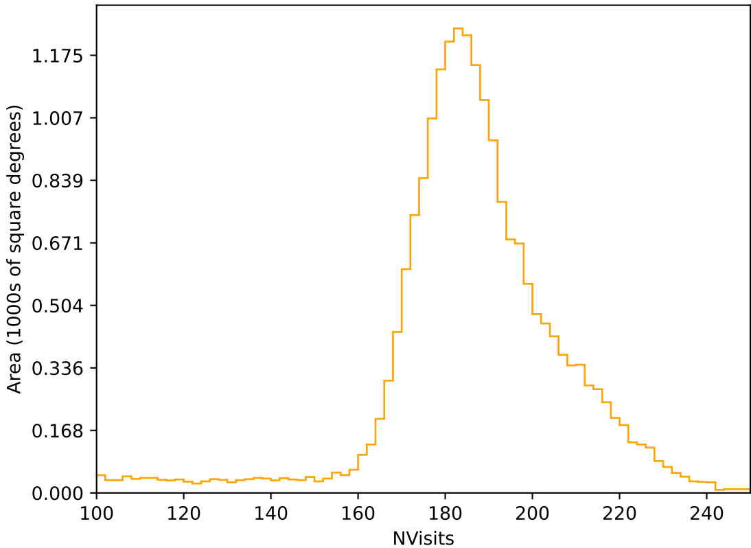
too_elab_heavy_r32_d3_gz_v3.4_10yrs All sky r band: NVisits
