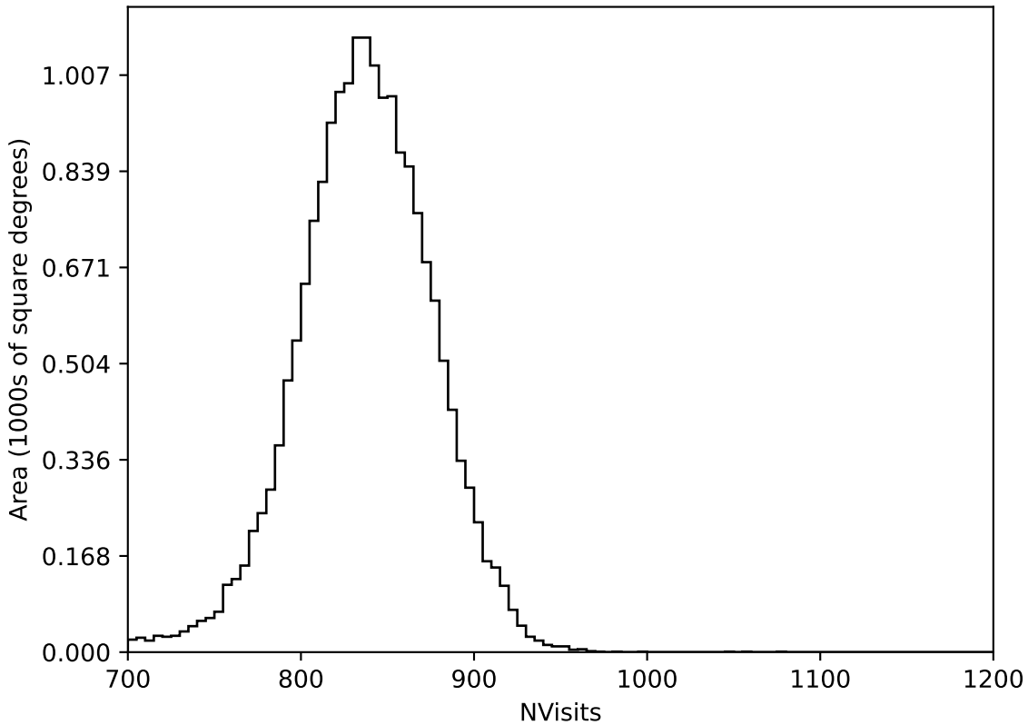
too_elab_heavy_r32_d3_gz_v3.4_10yrs All sky all bands: NVisits
