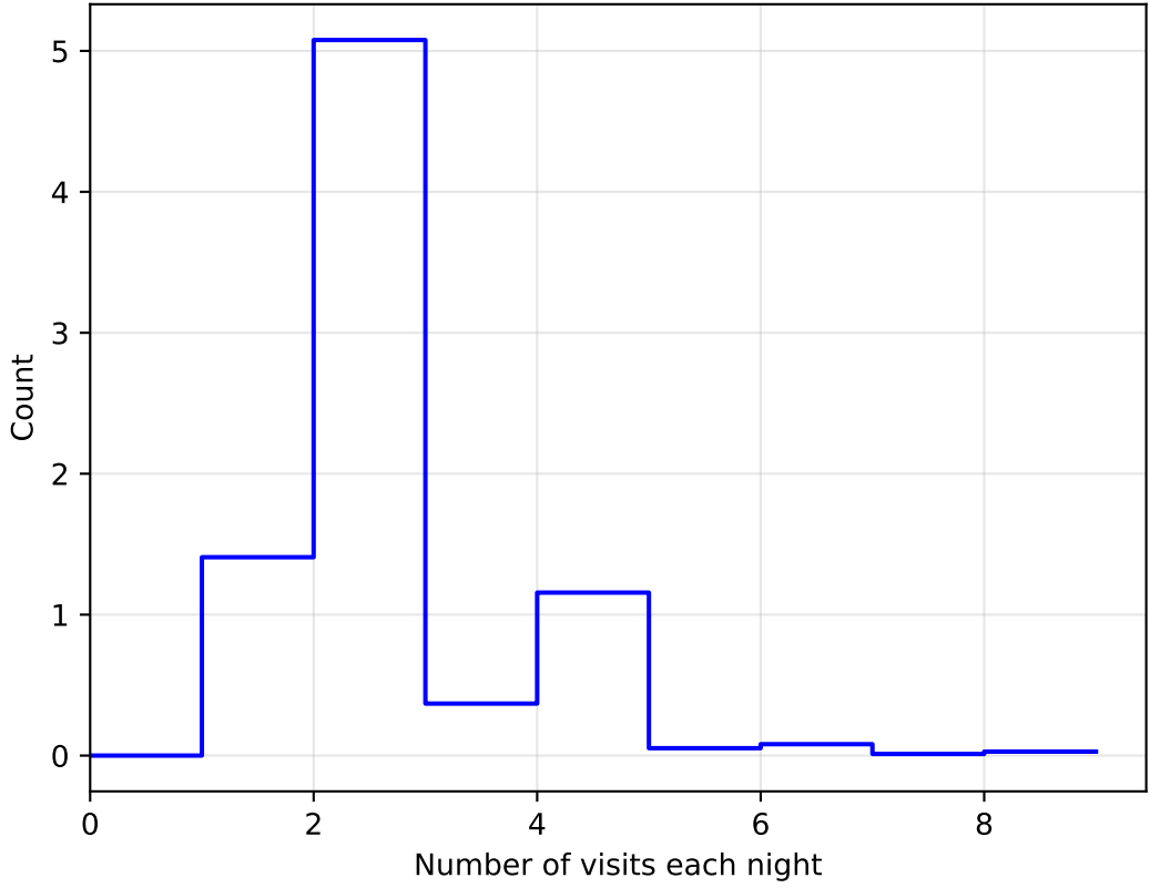
too_elab_heavy_r32_d3_gz_v3.4_10yrs WFD: NVisitsPerNight 1e6
