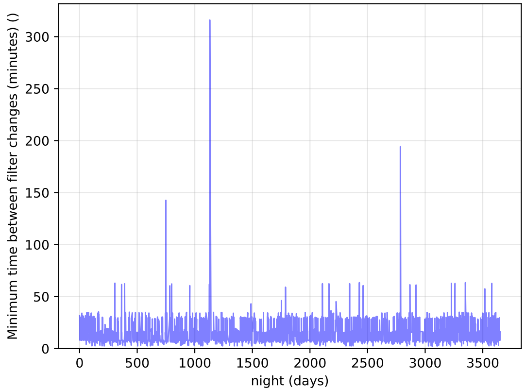
too_elab_heavy_r32_d3_gz_v3.4_10yrs Per Night: Minimum time between filter changes (minutes)
