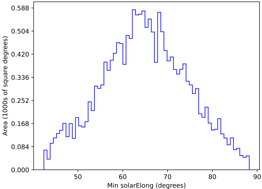
too_elab_heavy_r32_d3_gz_v3.4_10yrs WFD y band: Min solarElong
